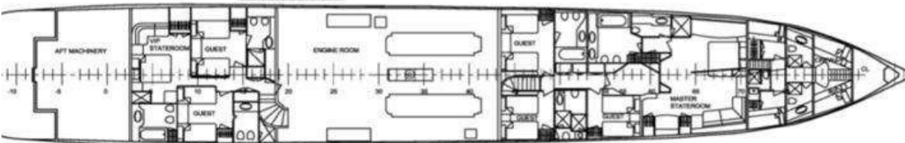
LOWER DECK
