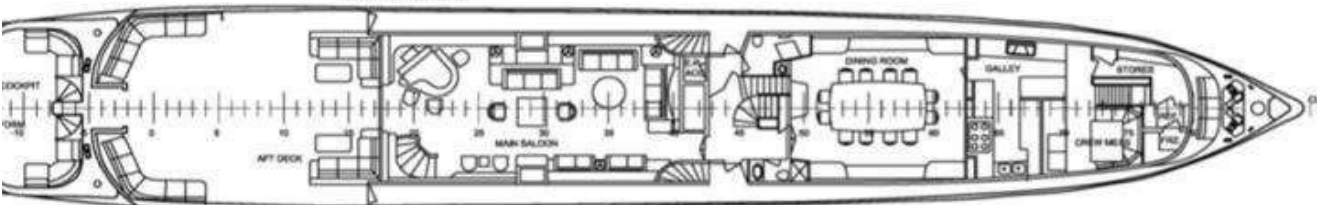
MAIN DECK
